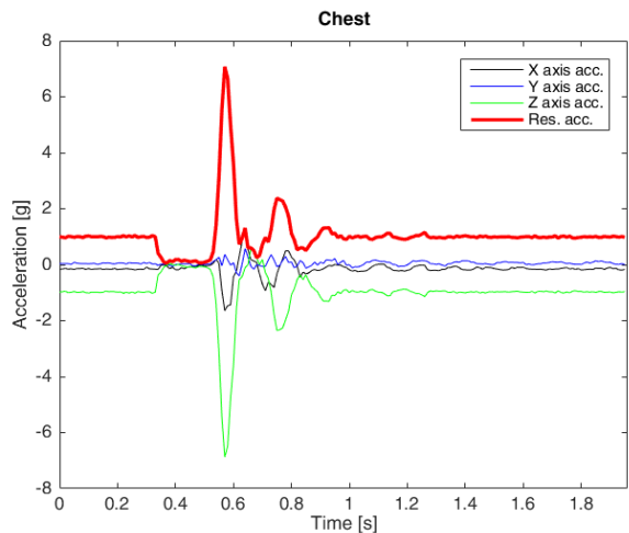
Fig. 7. Profile of registered acceleration values in the dummy chest/neck with the calculated resultant value – TEST 3
