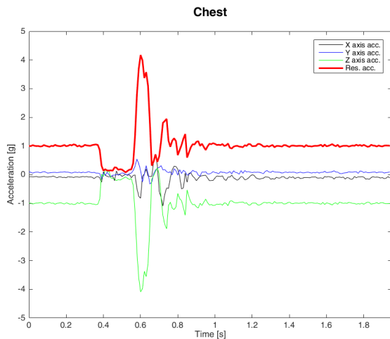
Fig. 11. Profile of registered acceleration values in the dummy chest/neck with the calculated resultant value – TEST 5
