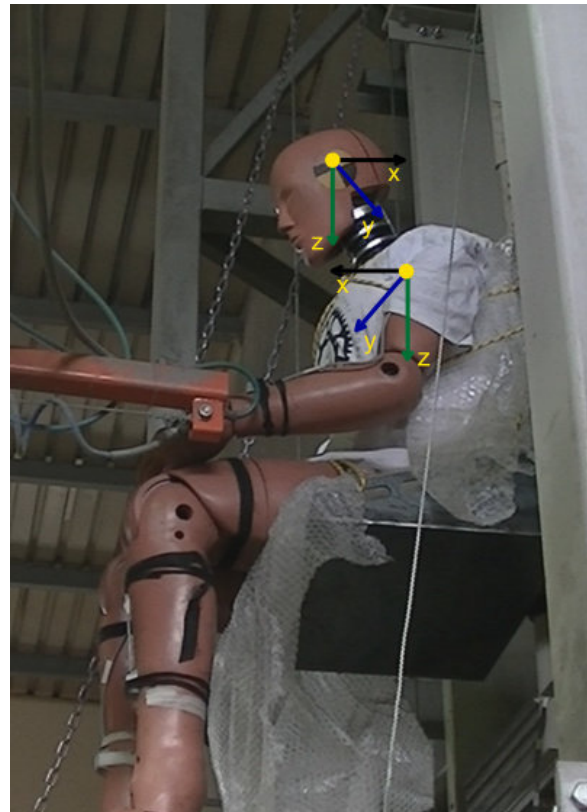
Fig. 12. The dummy with marked axes of head and chest accelerometers
