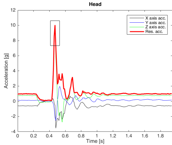
Fig. 4. Profile of registered acceleration values in the dummy head with the calculated resultant value – TEST 2
