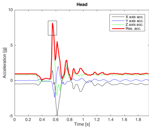
Fig. 6. Profile of registered acceleration values in the dummy head with the calculated resultant value – TEST 3
