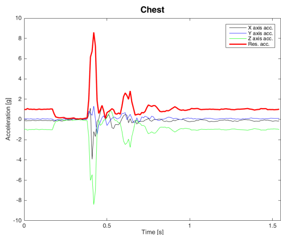
Fig. 3. Profile of registered acceleration values in the dummy chest/neck with the calculated resultant value – TEST 1
