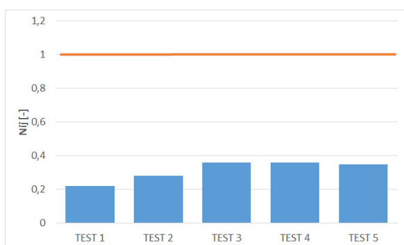
Fig. 14. The values of Nij index obtained during individual emergency braking tests with the limit value marked
