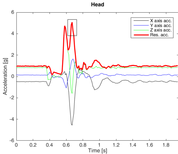
Fig. 10. Profile of registered acceleration values in the dummy head with the calculated resultant value – TEST 5
