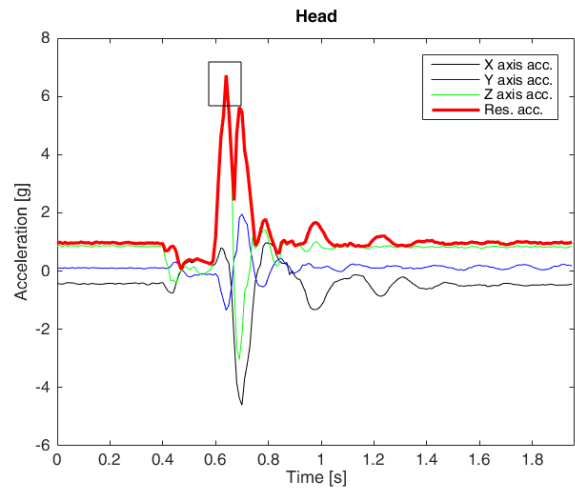
Fig. 8. Profile of registered acceleration values in the dummy head with the calculated resultant value – TEST 4
