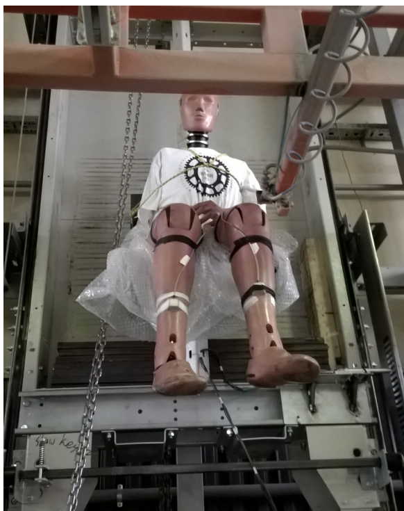
Fig. 1. The test dummy Hybrid III placed on the measuring site
