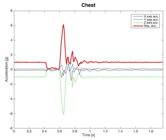
Fig. 9. Profile of registered acceleration values in the dummy chest/neck with the calculated resultant value – TEST 4
