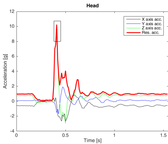
Fig. 2. Profile of registered acceleration values in the dummy head with the calculated resultant value – TEST 1
