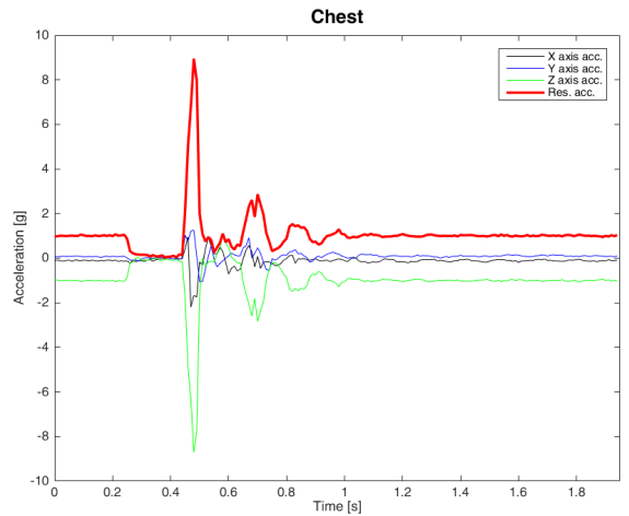
Fig. 5. Profile of registered acceleration values in the dummy chest/neck with the calculated resultant value – TEST 2
