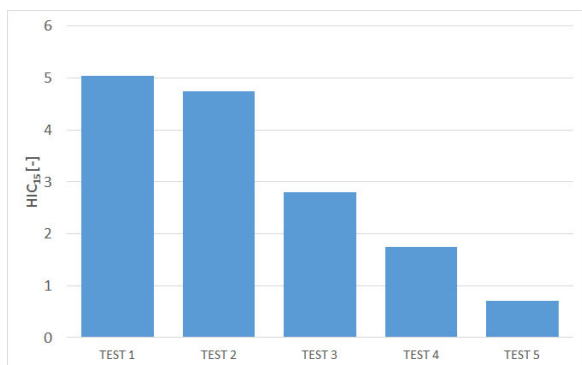
Fig. 13. The values of HIC index obtained during individual emergency braking tests
