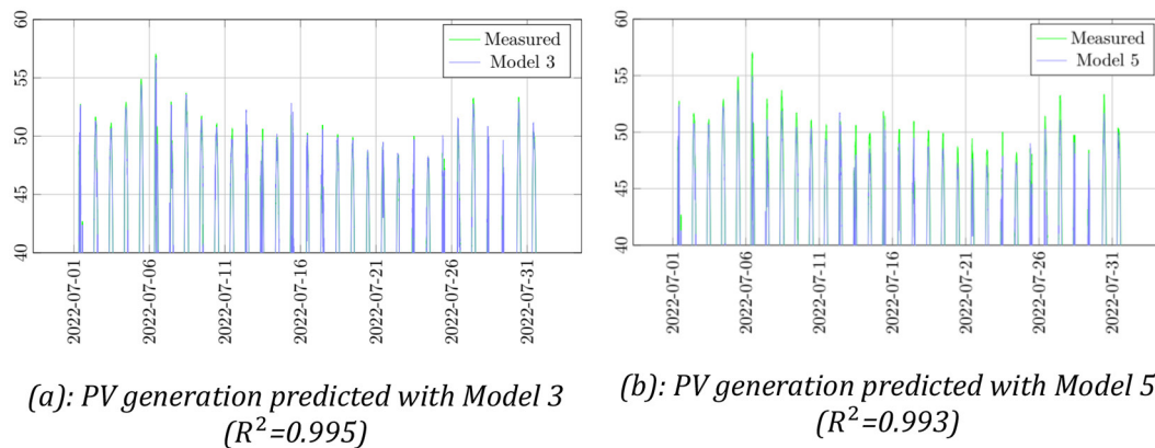
Figure 7. Prediction results of PV generation for example month (2022-07)
