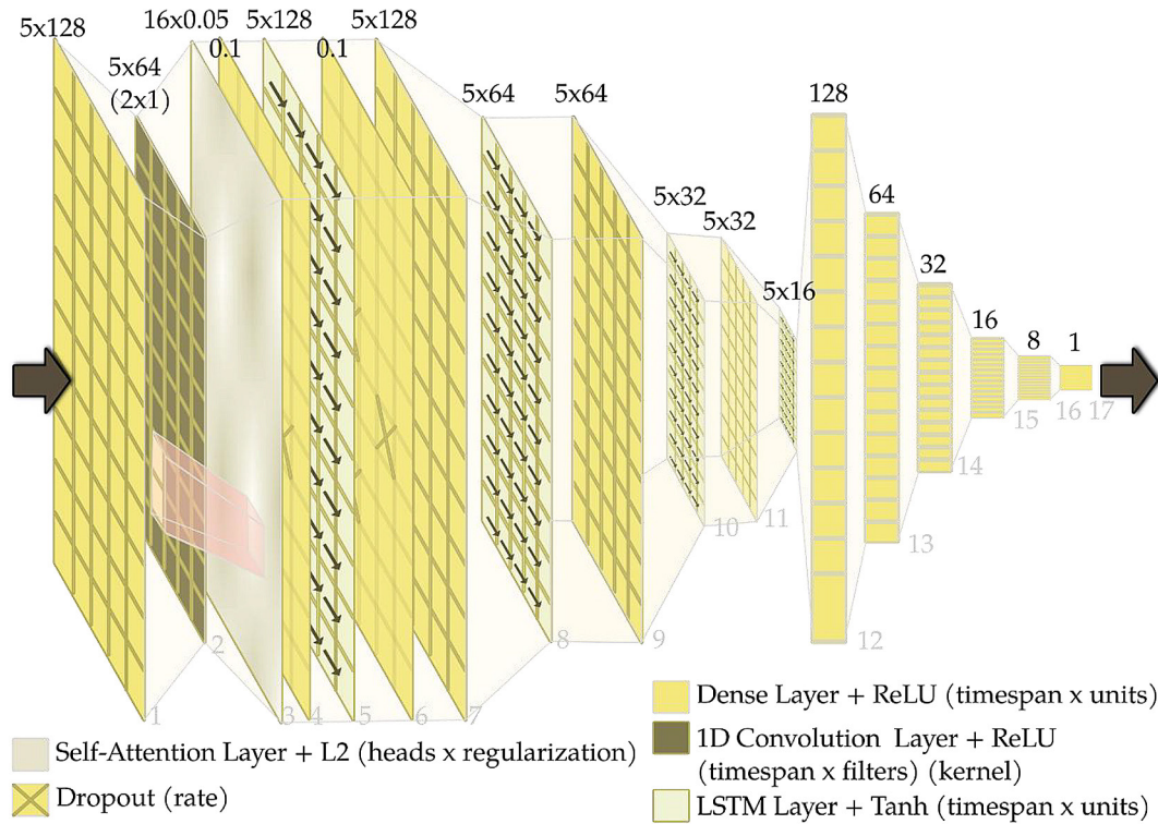
Figure 2. The proposed neural network architecture. Network consists of three types of layers: Dense, Recurrent and Convolutional. The first part of the network works on temporal data with time span of 5 min. Temporal data are flattened in the last recurrent layer with do not return each sequences. Second part of the network consists of only dense layers (time span = 1). The Self-Attention layer consists of Multi Head Attention with 16 heads, addition layer and normalization layer
