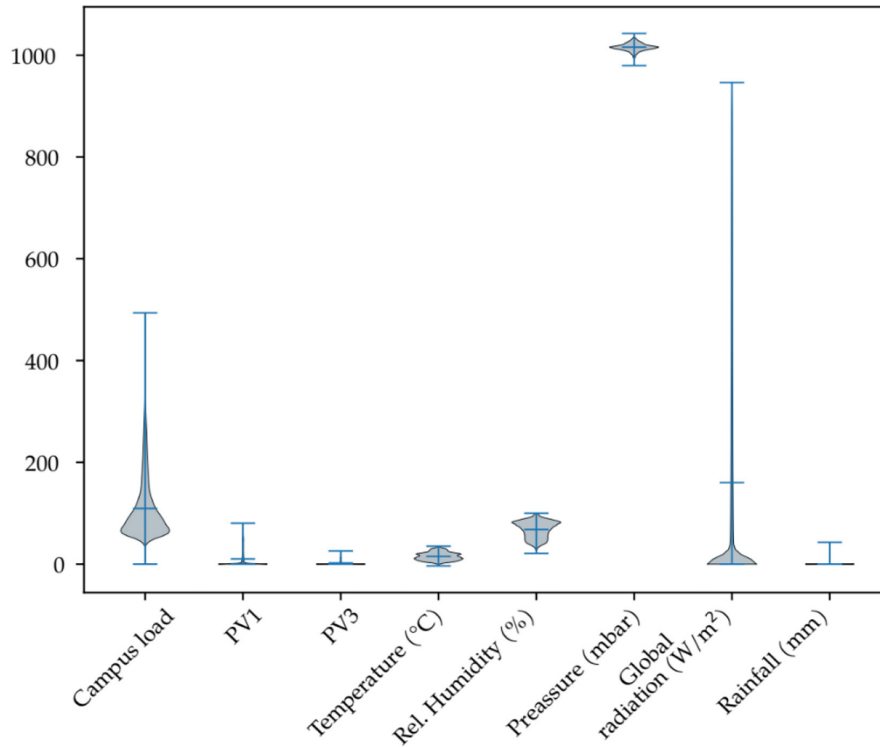
(a): Distribution of analyzed features
