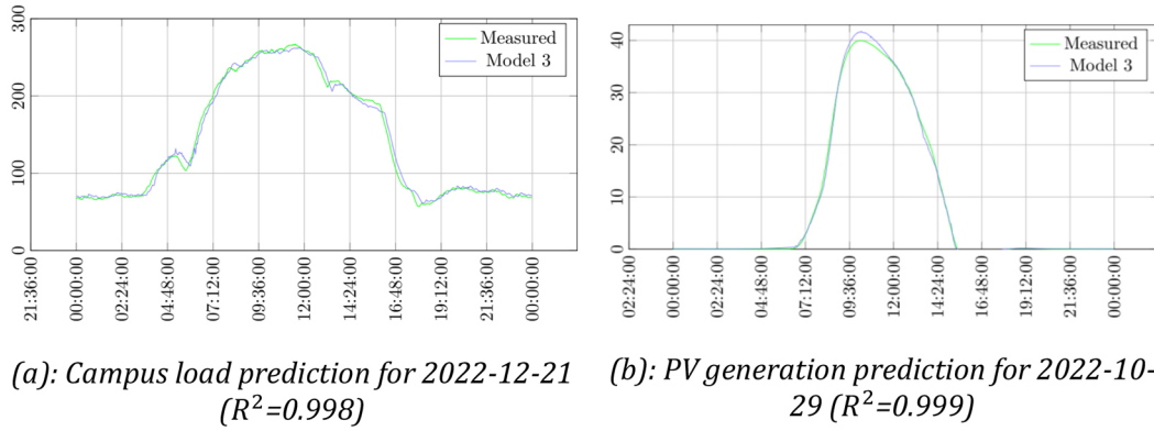
Figure 8. Prediction results of example day with Model 3
