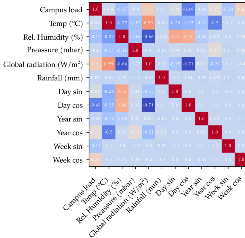
(b): Correlation matrix of analyzed features
