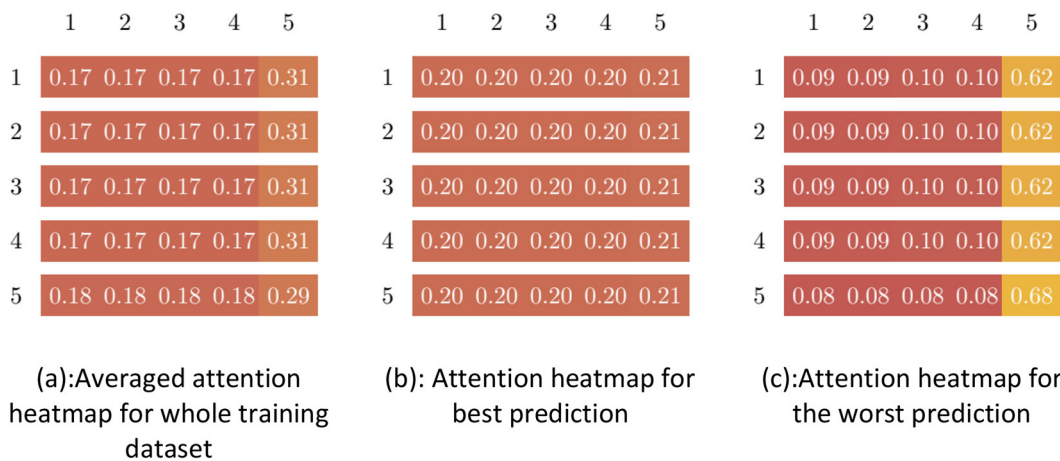
Figure 10. Analysis of the self-attention layer heatmap
