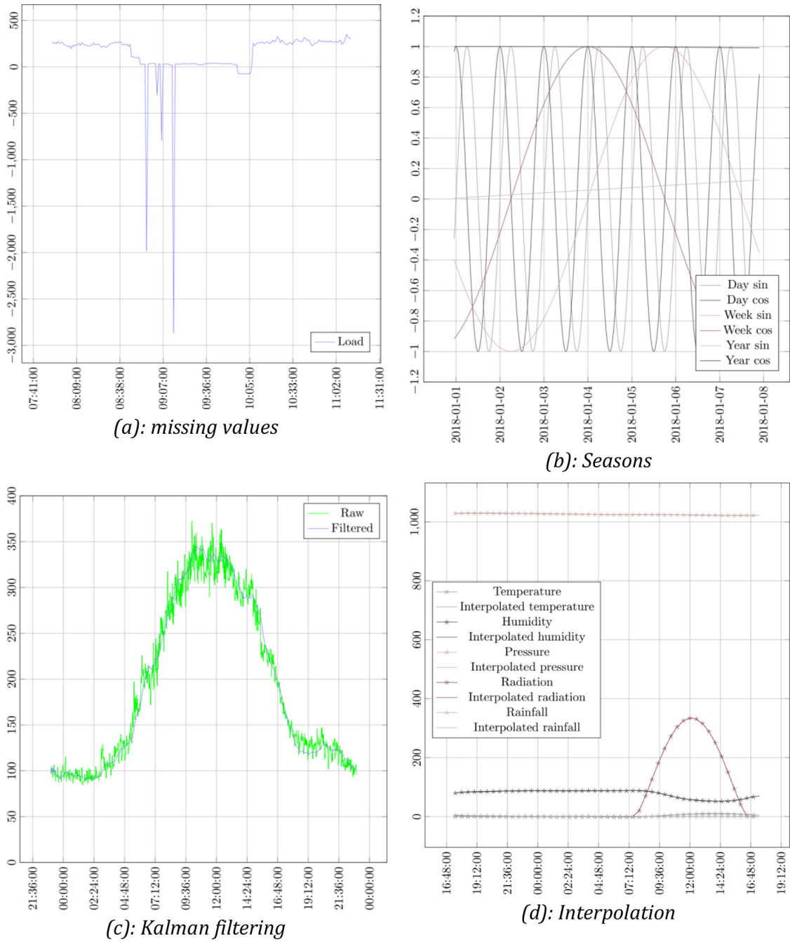
Figure 3. Preprocessing tasks
