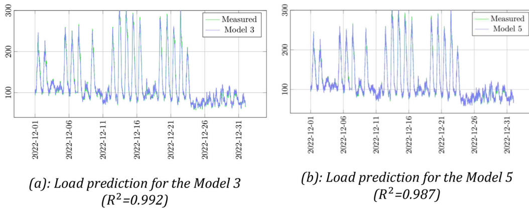
Figure 6. Prediction results of campus load for the example month (2022-12)
