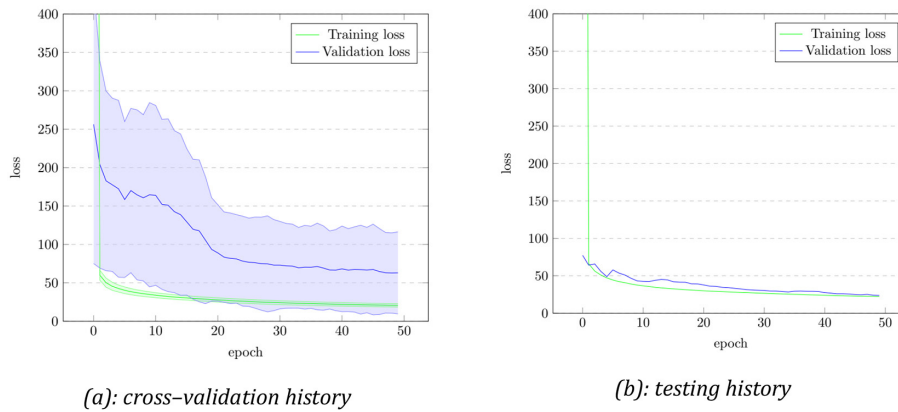
Figure 5. Loss curve for training the model number 3 with Kalman filter and LSTM layers
