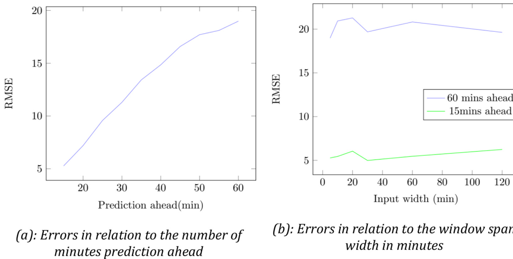
Figure 9. Analysis of the influence of the model parameters on produced errors in predicting campus load
