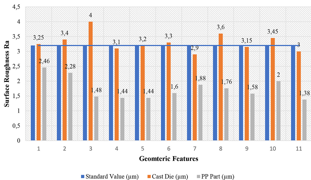
Figure 9. Surface roughness comparison
