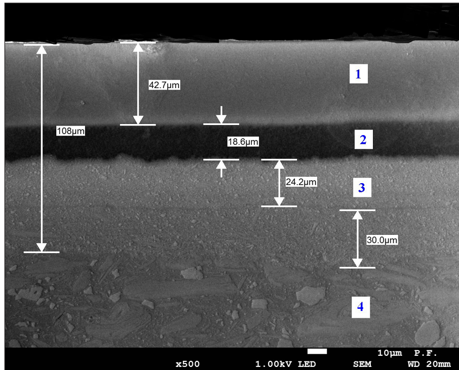
Figure 2. SEM image of the polished cross-section through an anti-graffiti BO100-AGR coating system on steel substrate: 1 – anti-graffiti layer, 2 – base layer, 3 – undercoat layer, 4 – putty
