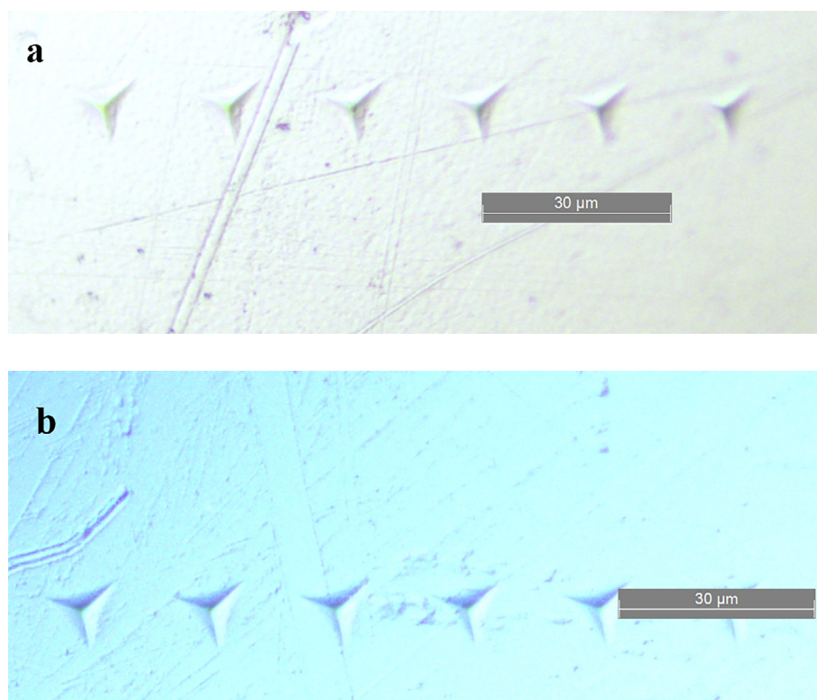
Figure 10. Indentation marks during nanohardness measurements on the surface of anti-graffiti paint coating: a) BO100-AGR, b) XPC 60036
