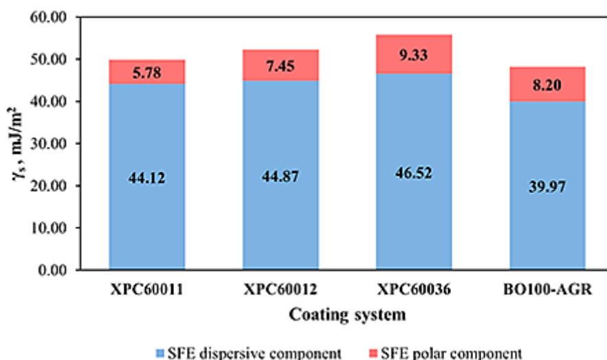
Figure 4. Comparison of the components of the total surface energy of the tested systems anti-graffiti coatings
