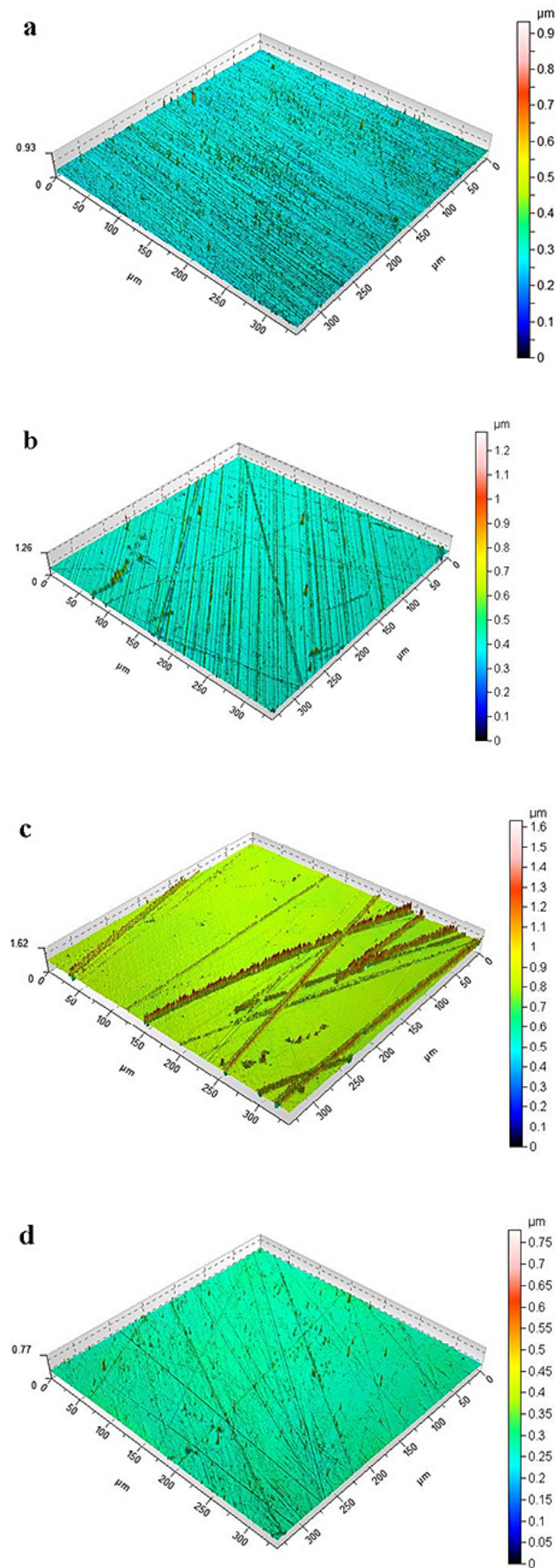
Figure 8. Surface roughness for the anti-graffiti coatings: a) XPC 60012, b) XPC 60036, c) XPC 60011, d) BO100-AGR
