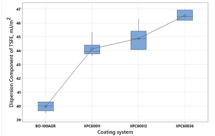
Figure 6. Distribution of the dispersive component of the total surface free energy DC-TSFE values
