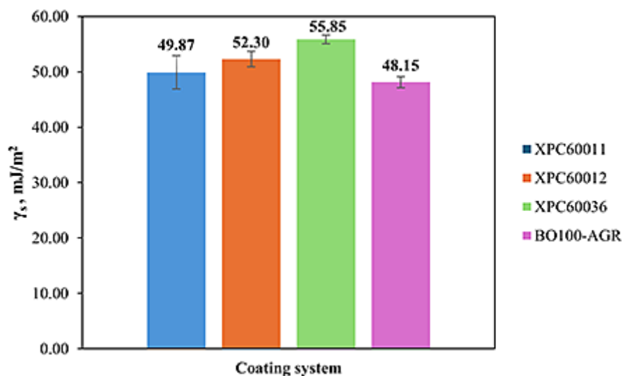
Figure 3. Comparison of the total surface free energy of the tested systems anti-graffiti coatings
