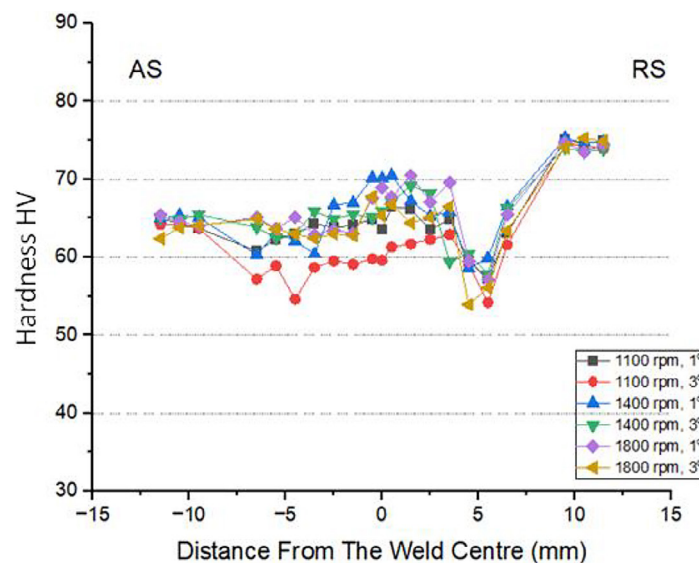
Figure 8. MicroVickers hardness measurement
