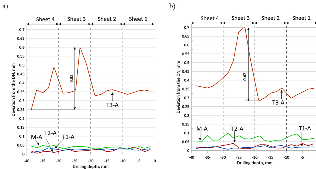
Figure 5. Deviation of actual diameter from nominal diameter. (a) configuration A in package sheet 1, (b) configuration A in package sheet 2; volumetric efficiency VE = 39.8 \text{ cm}^3/\text{min}
