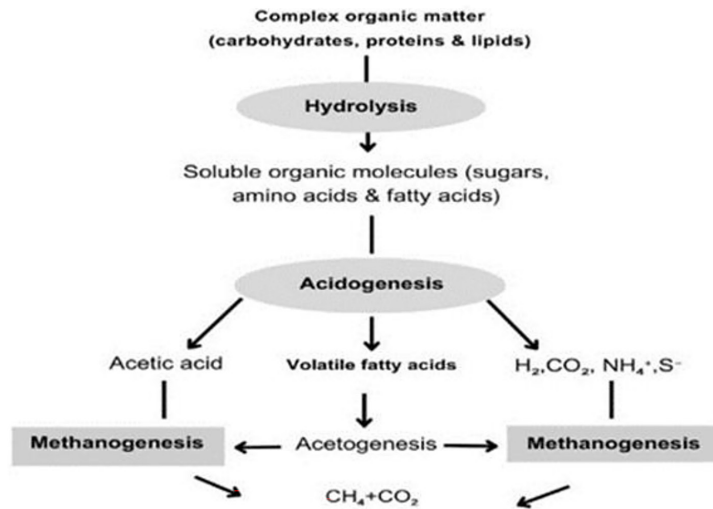
Figure 1. Stages of anaerobic digestion (methane fermentation process) [21]
