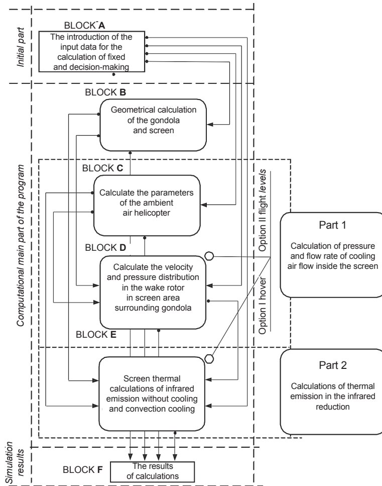
Fig. 9. Block schematic of calculation programme INFRED-EKRAN_1_0.exe, Part 2 written in Fortran 95 language
