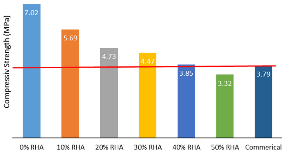
Fig. 4. Comparison of 28 days compressive strength
