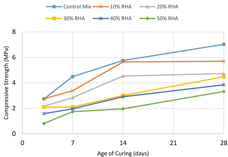
Fig. 2. Variation of compressive strength of blocks with age of curing
