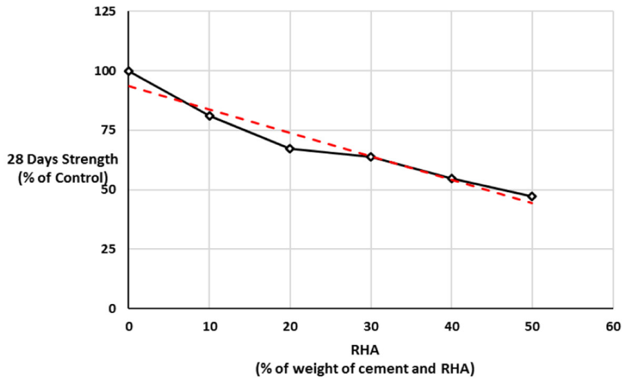
Fig. 3. Percentage decrease in compressive strength with addition of RHA
