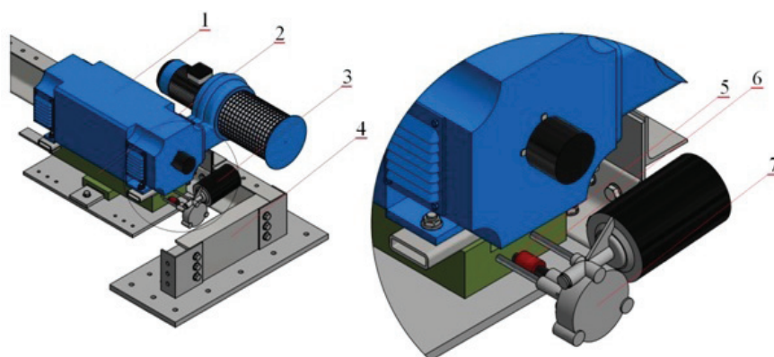
Fig. 5. Realization method of the increase the distance between rotors: 1 – DC motor used as brake, 2 – guide ways, 3 – electric motor with worm gear and lead screw, 4 – station’s frame, 5 – lead screw, 6 – coupling, 7 – worm gear
