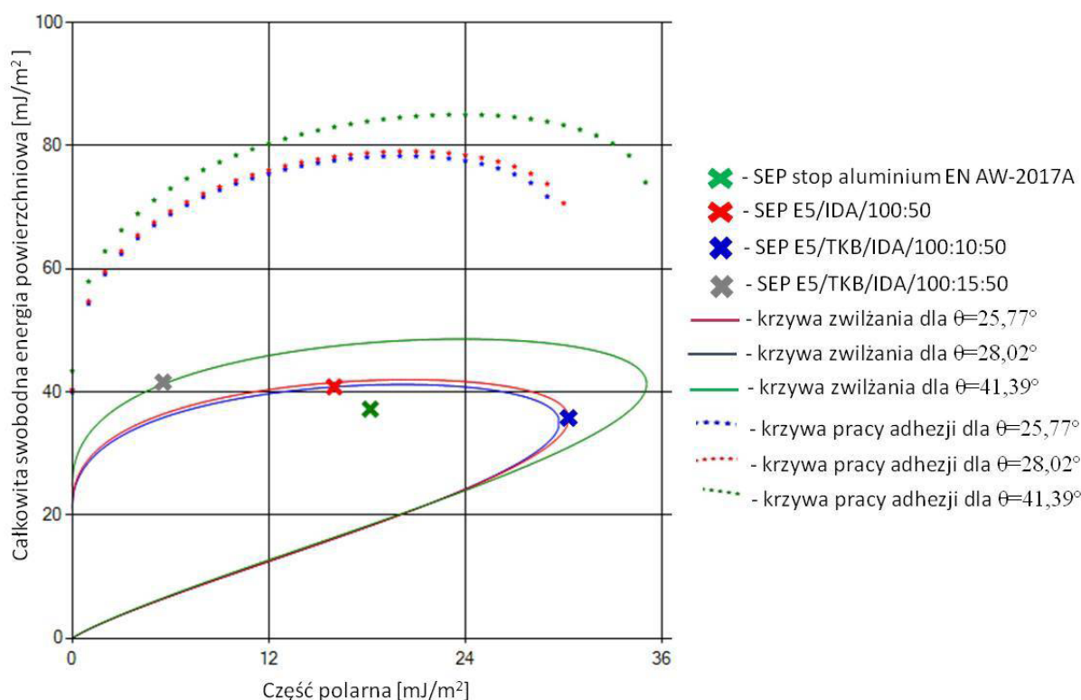
Fig. 3. Wetting envelopes and curves of work of adhesion determined for EN AW-2017A aluminium alloy and surface free energy values of selected adhesive compositions (prepared by the authors)
