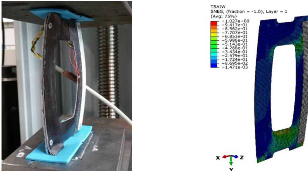
Fig. 7. Comparison of the a) experimental and b) numerical results for [45/-45/90/0]s
