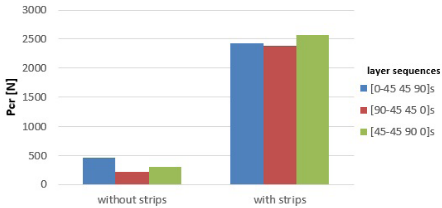
Fig. 8. The influence of stiffeners on the critical force
