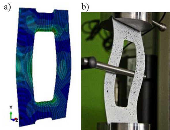
Fig. 1. Higher, flexural-torsional form of plate with cut-out loss of stability in the arrangement of [0/-45/45/90]s composite layers: a) FEM calculations - stable form, b) experimental research– unstable form (jump phenomenon)
