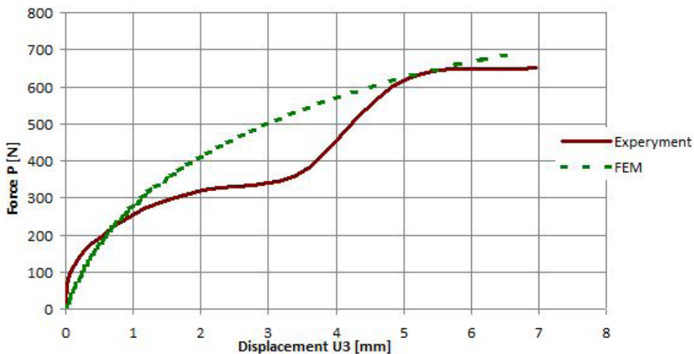
Fig. 2. Comparison of post-buckling paths appointed with FEM and experiment
