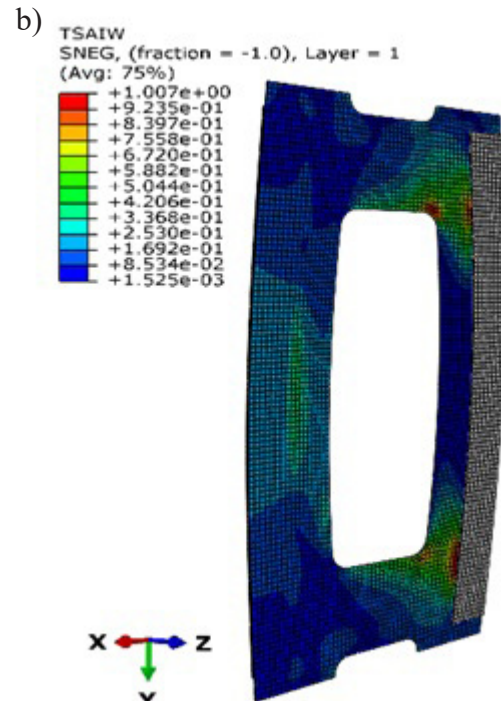
Fig. 6. Comparison of the a) experimental and b) numerical results for [0/-45/45/0]_s
