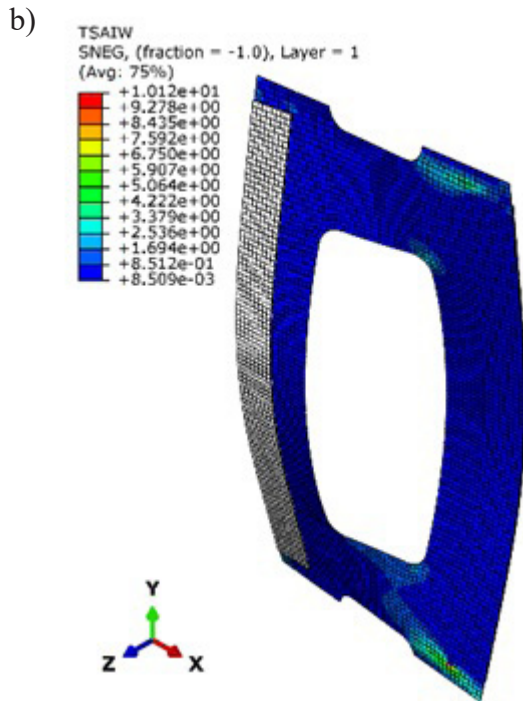
Fig. 5. Comparison of the a) experimental and b) numerical results for [90/-45/45/0]_s
