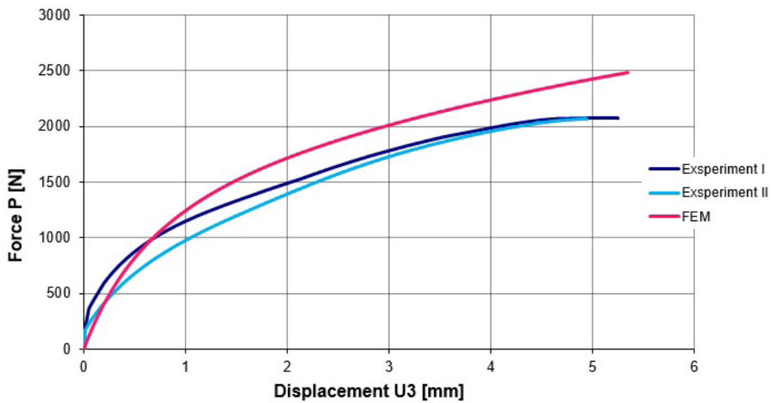
Fig. 9. Comparison of the experimental and numerical results for plate with [90/-45/45/0]s layer sequences
