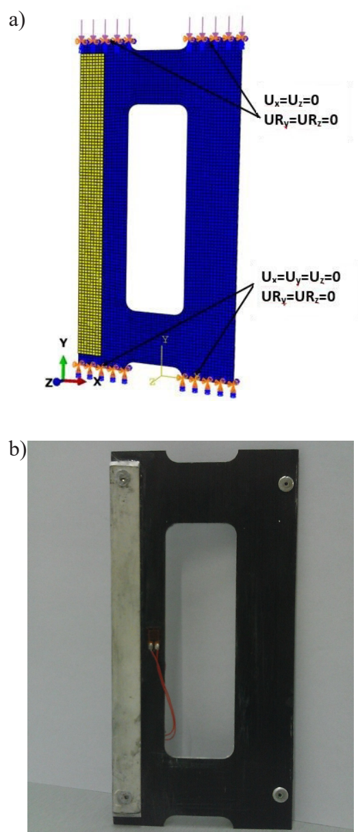
Fig. 3. Model of the tested composite plate with stripes a) numerical model with boundary conditions, b) real model
