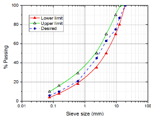
Figure 1. Aggregate gradation curve
