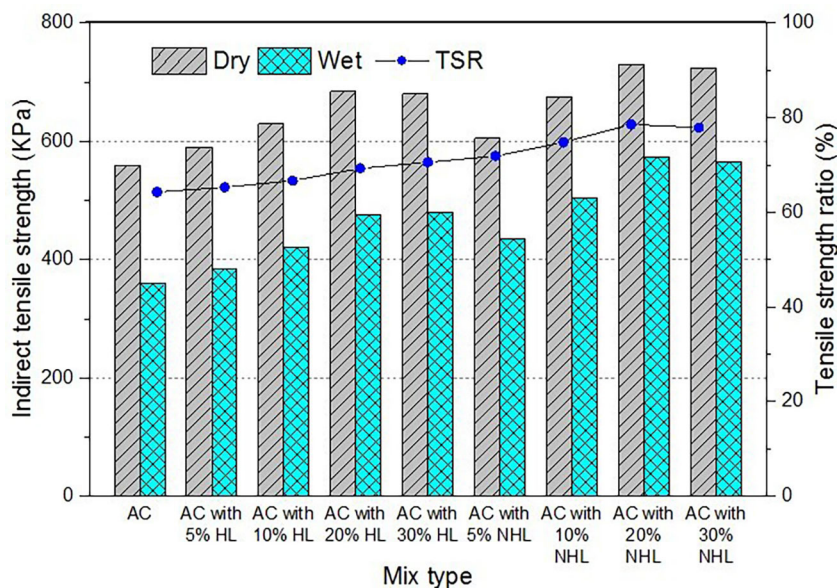
Figure 2. ITS and TSR results of mixtures with and without additives at wet and dry conditions
